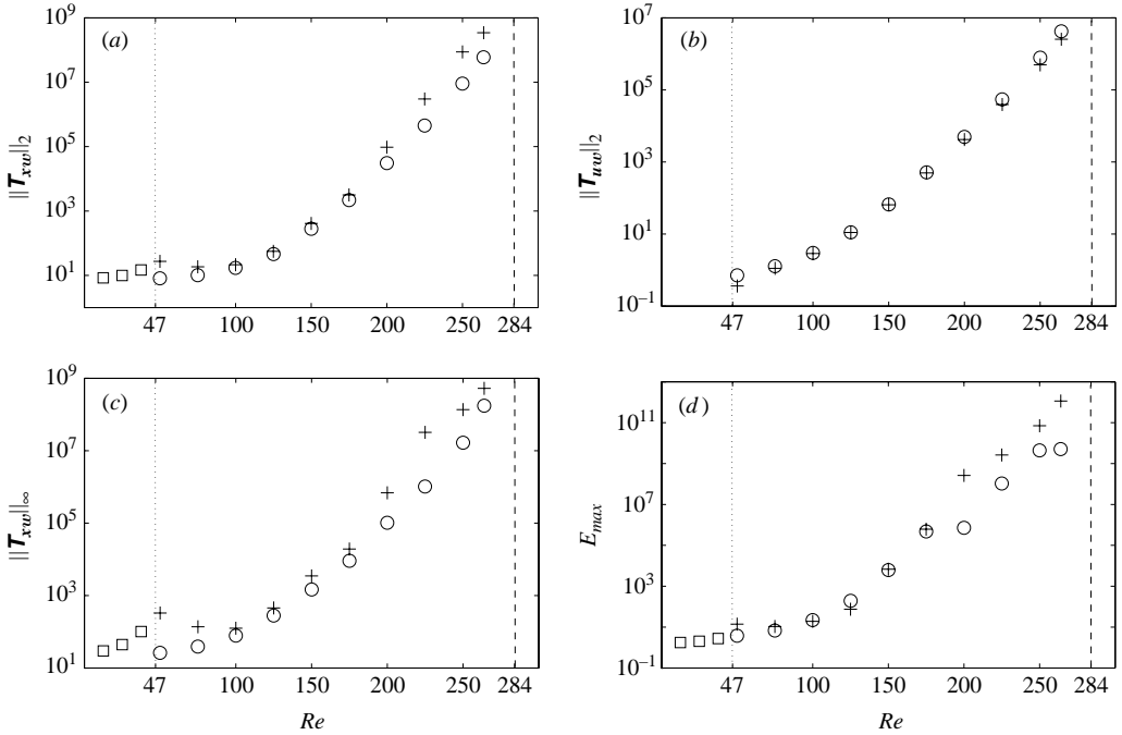
FIGURE 4. Performance of the uncontrolled ( \square , Re < 47 ) and controlled linear wake model as a function of Reynolds number for two control penalties (+) \ell = 1000 , (o) \ell = 0.1 using full information \mathcal{H}_2 control. (a) Transfer function 2-norm \|\mathbf{T}_{xw}\|_2 ; (b) transfer function 2-norm \|\mathbf{T}_{uw}\|_2 ; (c) transfer function \infty -norm \|\mathbf{T}_{xw}\|_\infty ; (d) maximum transient energy growth E_{max} . All plots are semilog-y and were computed using double precision arithmetic; note that, at this precision, stabilizing linear control feedback could not be determined above Re \approx 284 .
